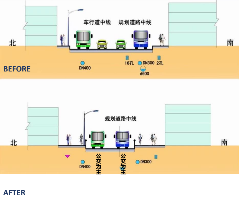
Eastern Section—Bus-oriented
